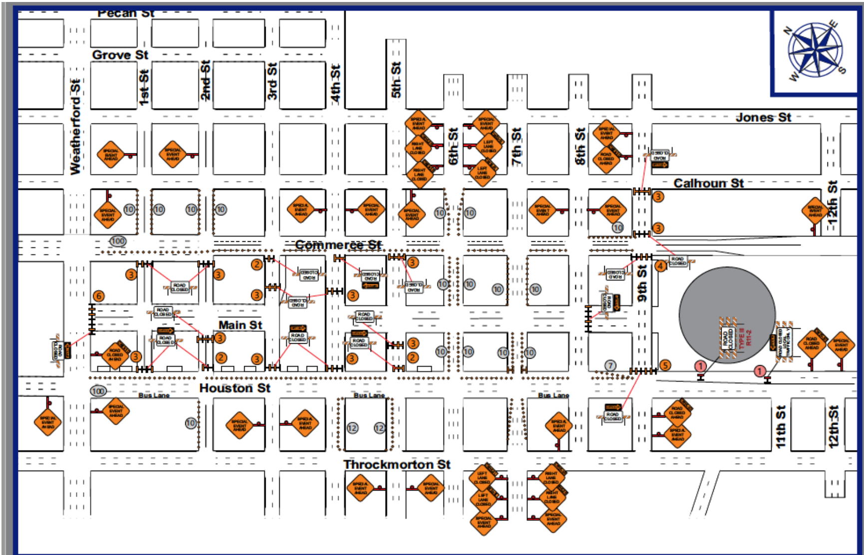
MAIN ST. Fort Worth Arts Festival 2025 TENTATIVE TUESDAY, 4/8/2025 TRAFFIC CONTROL PLAN
