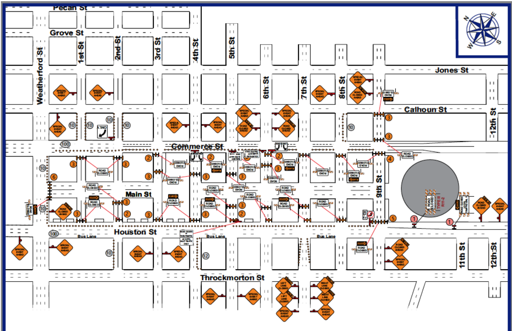
MAIN ST. Fort Worth Arts Festival 2025 TENTATIVE FRIDAY, 4/11/2025 TRAFFIC CONTROL PLAN
