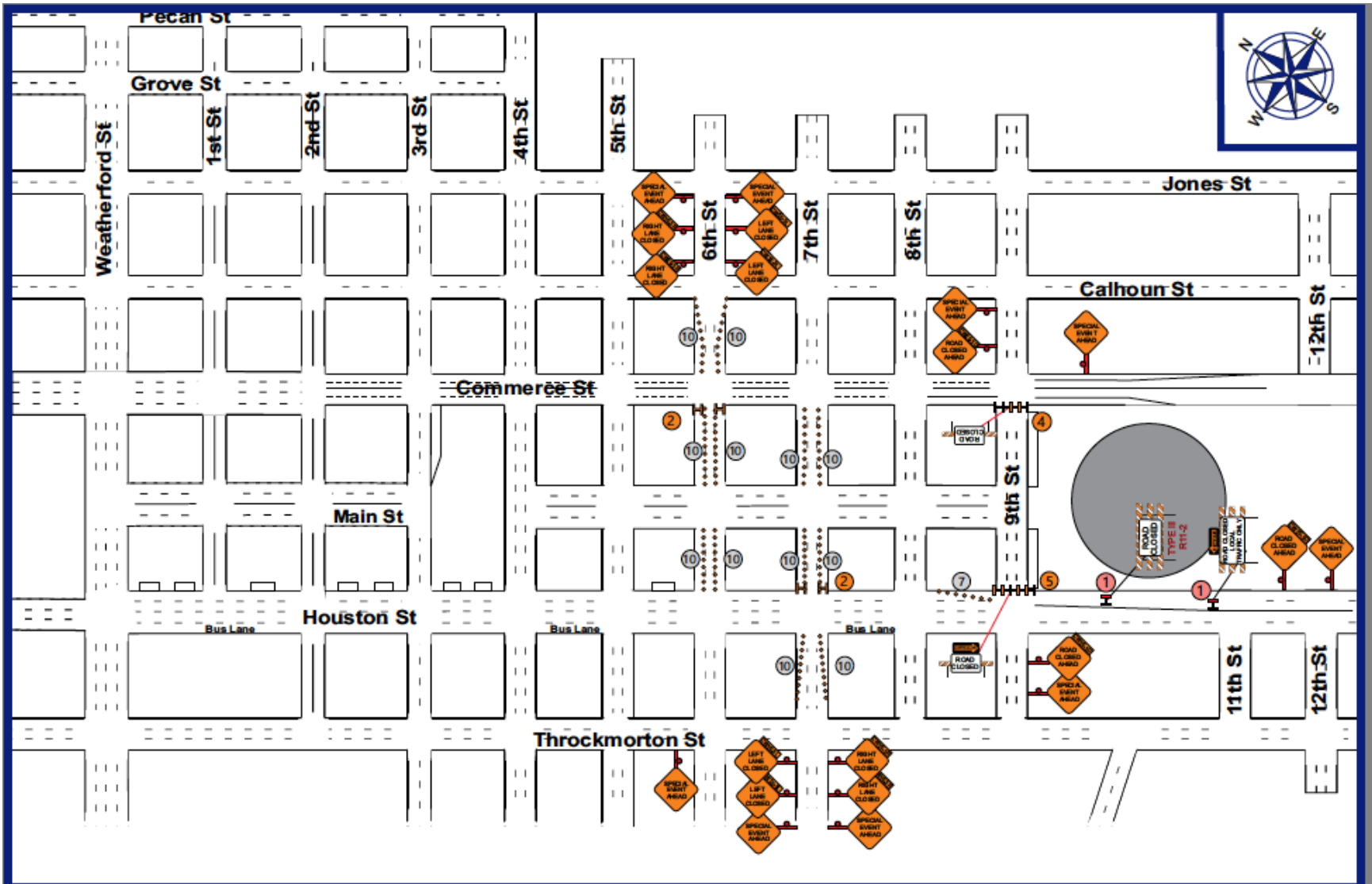
MAIN ST. Fort Worth Arts Festival 2025 TENTATIVE THURSDAY, 4/10/2025 TRAFFIC CONTROL PLAN
