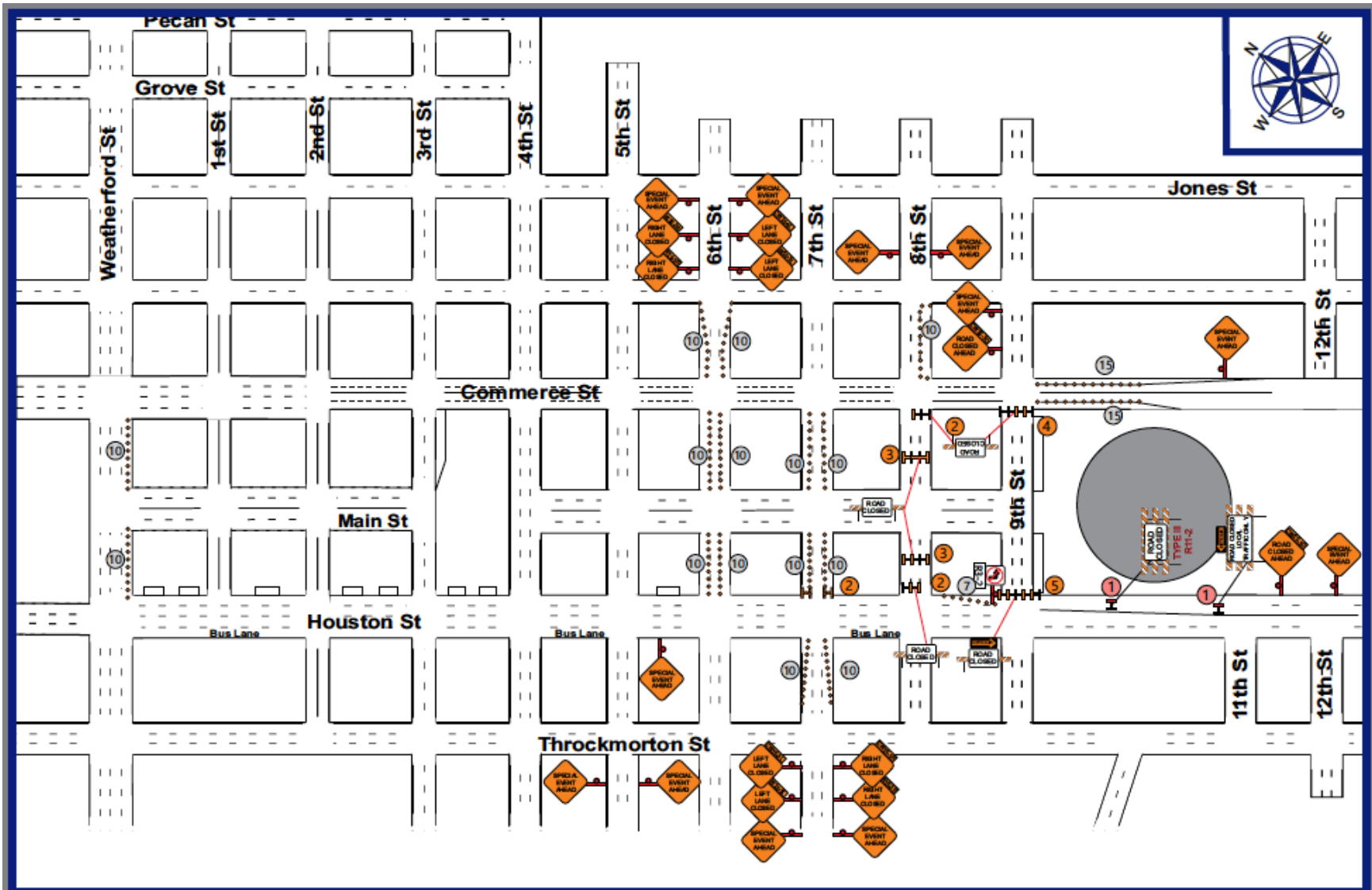
MAIN ST. Fort Worth Arts Festival 2025 TENTATIVE WEDNESDAY, 4/9/2025 TRAFFIC CONTROL PLAN
