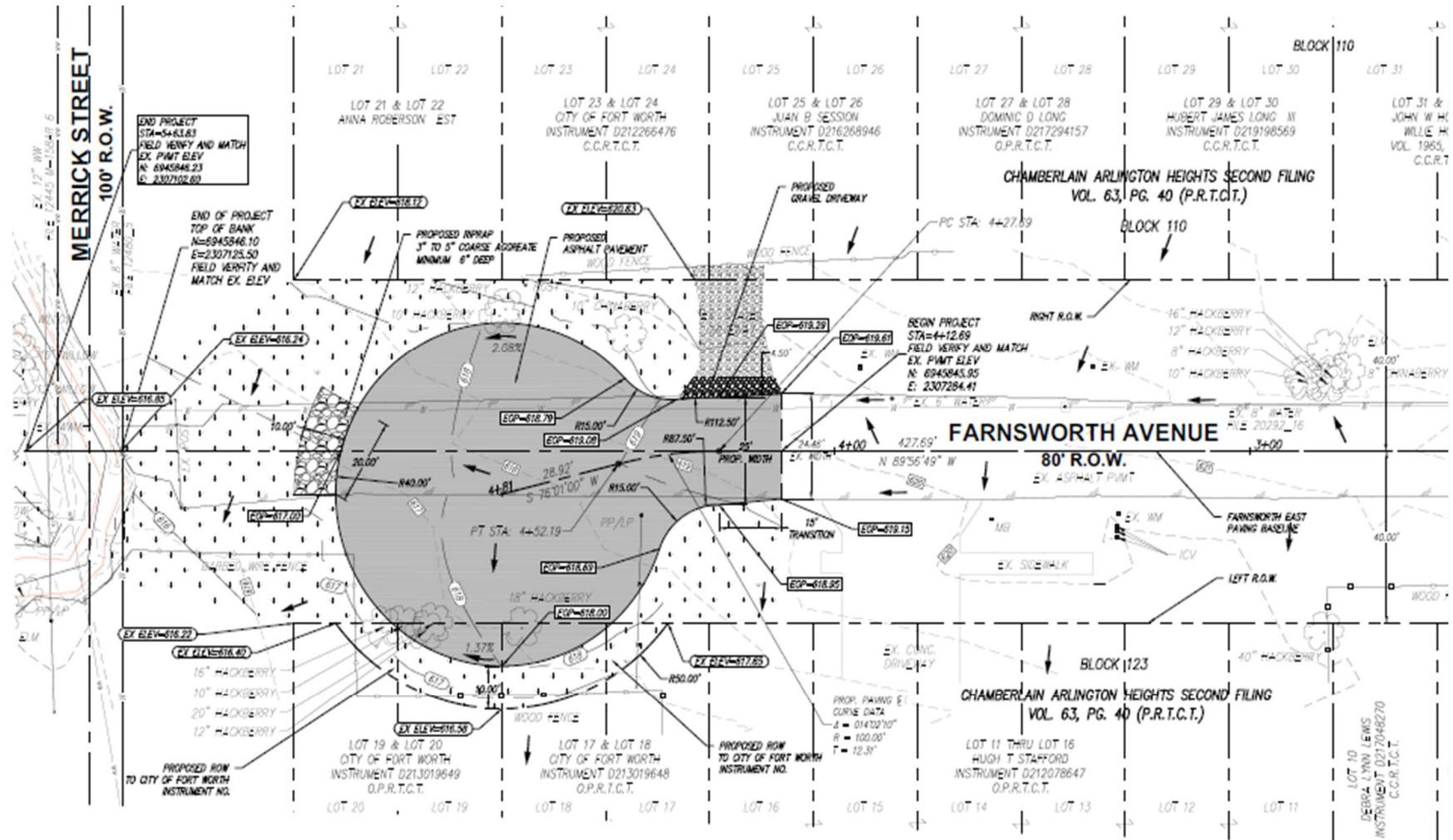
Cul-de-sac plans for the west side of the stream of Farnsworth Avenue
