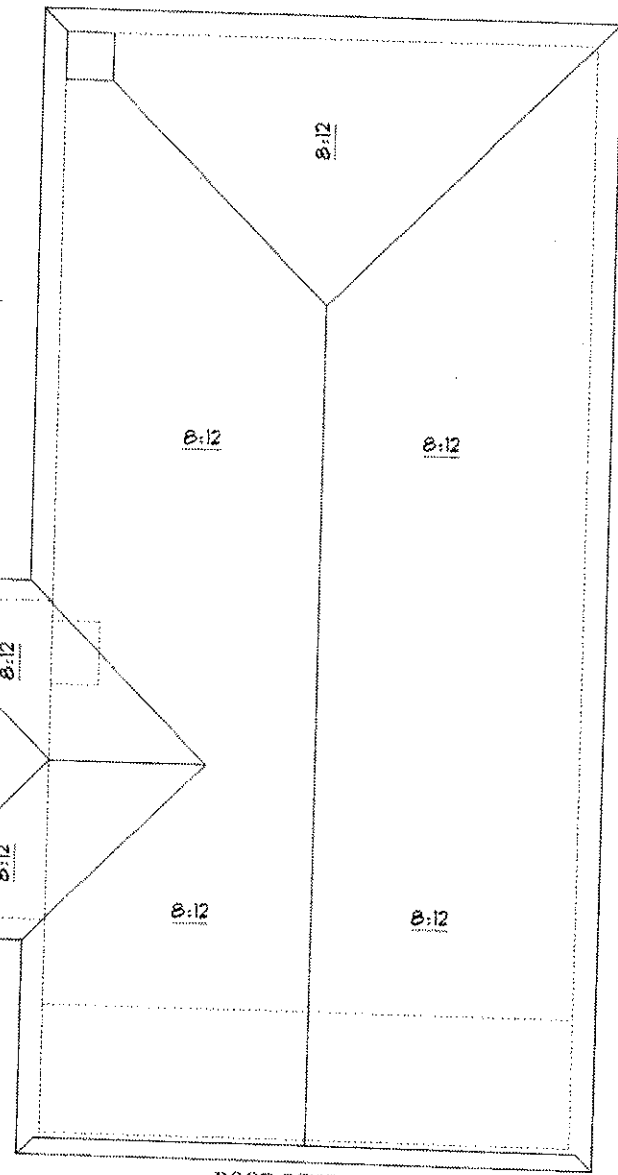
ROOF SCHEMATIC SCALE: 1/4" = 1'-0"
