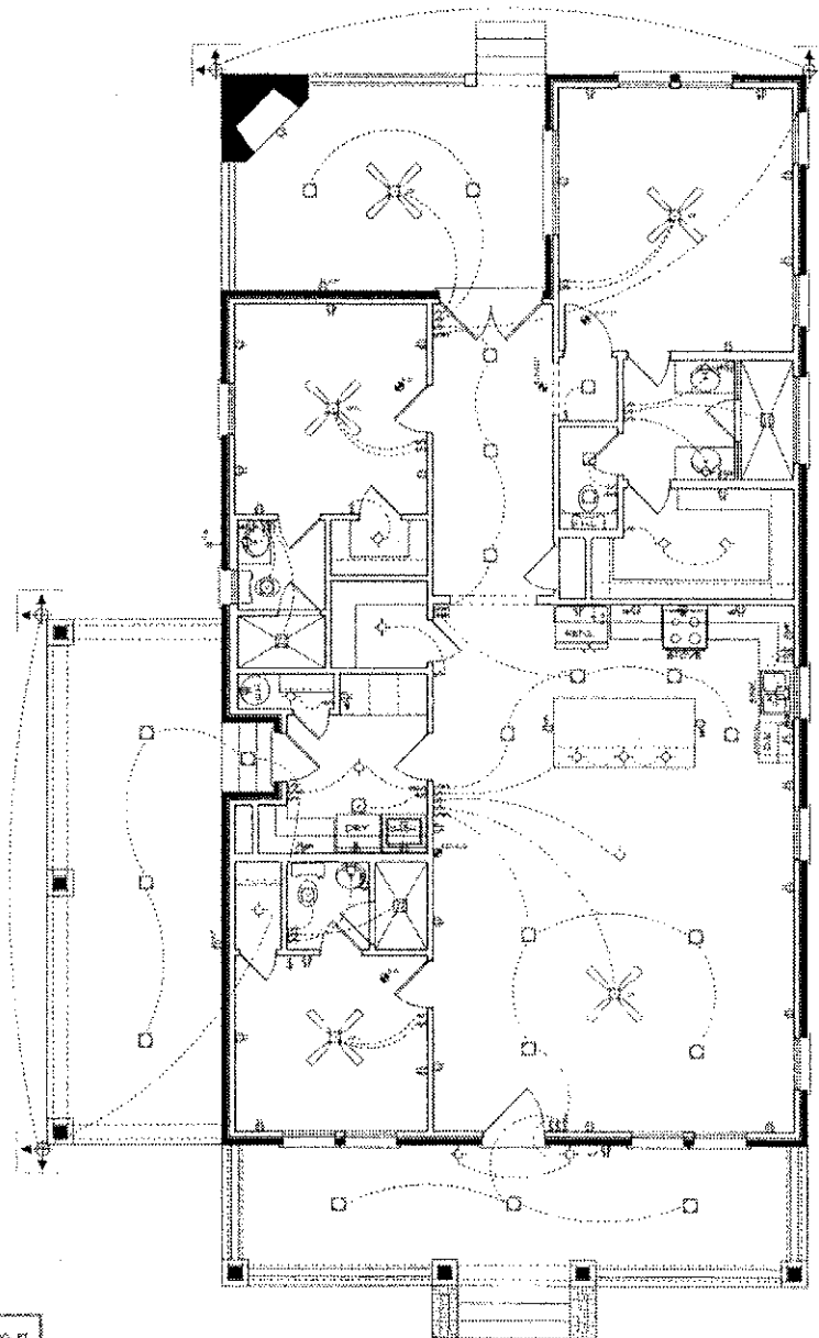
ELECTRICAL PLAN SCALE: 1/4" = 1'-0"
