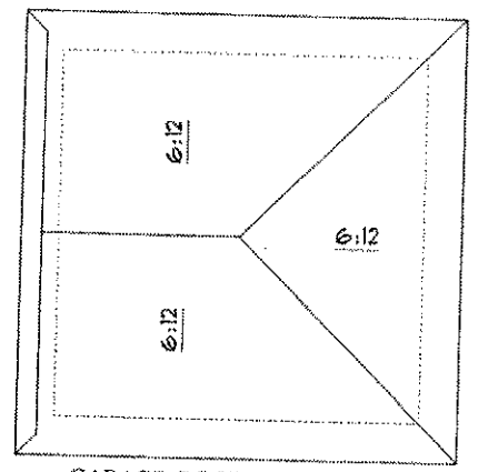
GARAGE ROOF SCHEMATIC SCALE: 1/4" = 1'-0"
