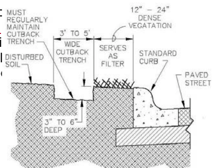
SECTION UNDERCUT LOT NOT TO SCALE
