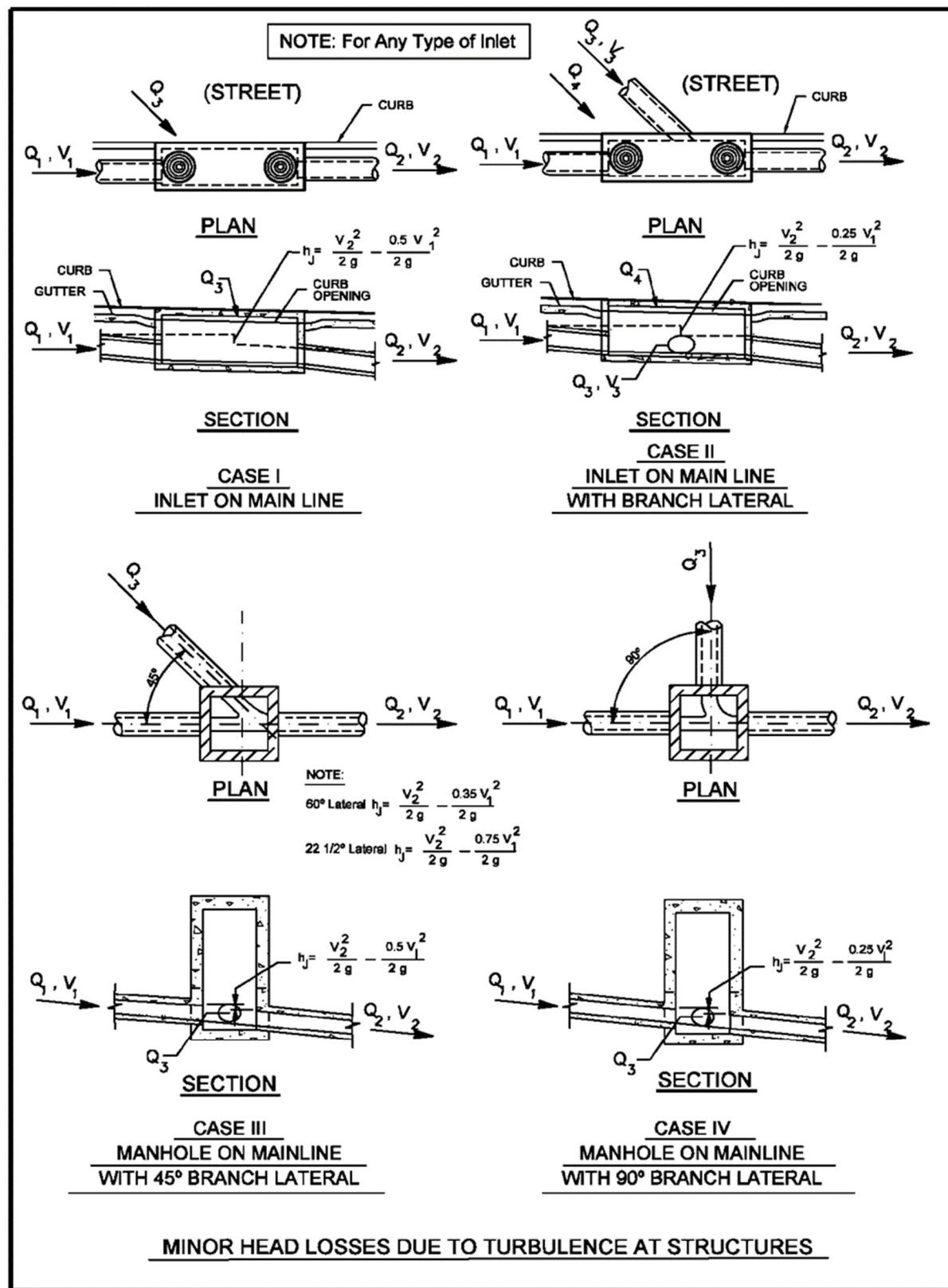
Figure 3-83.8 Minor Head Losses at Structures (1 of 2)
