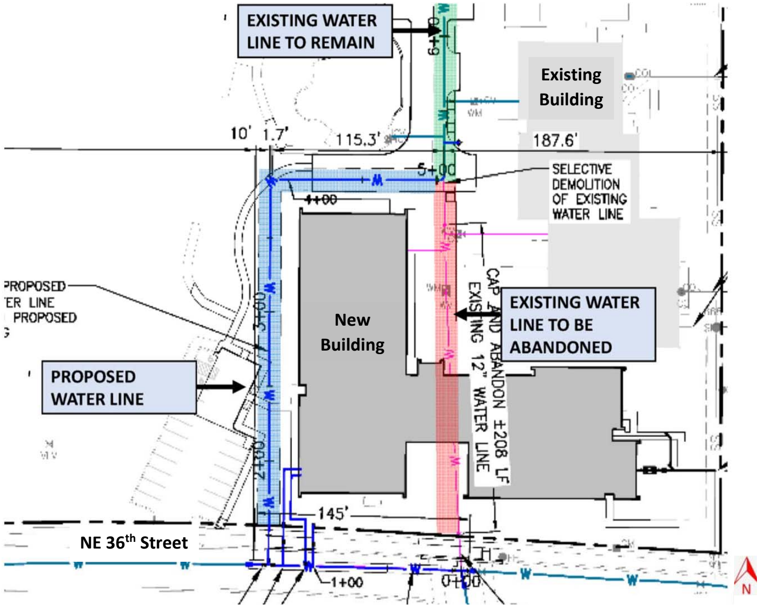
Existing and Proposed Water Line Location
