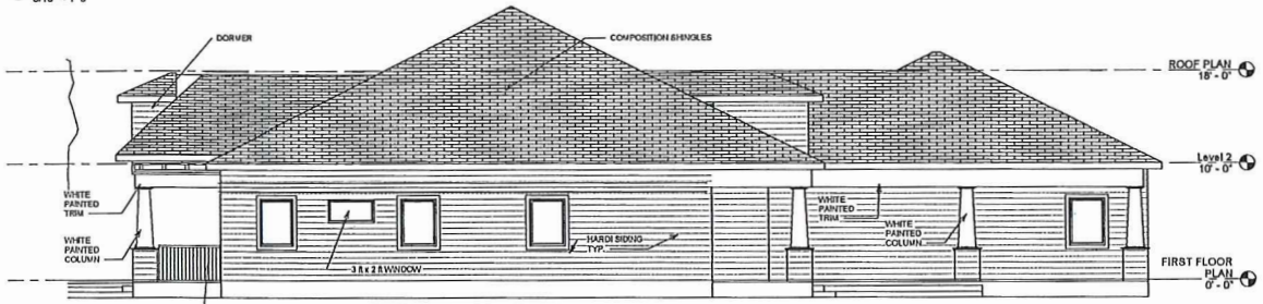
3 EAST ELEVATION 3/16" = 1'-0"
