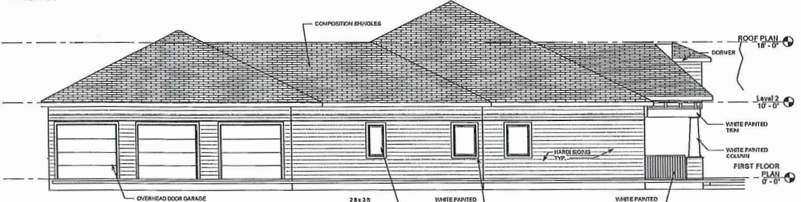
4 WEST ELEVATION 3/16" = 1'-0"
