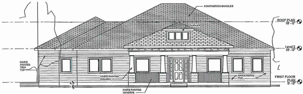
1 FRONT ELEVATION 3/16" = 1'-0"
